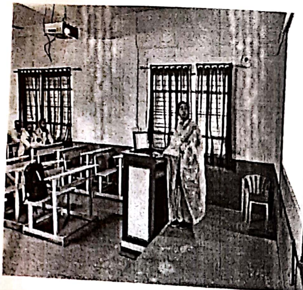
CHEMDRAW LECTURE 2017-18.
