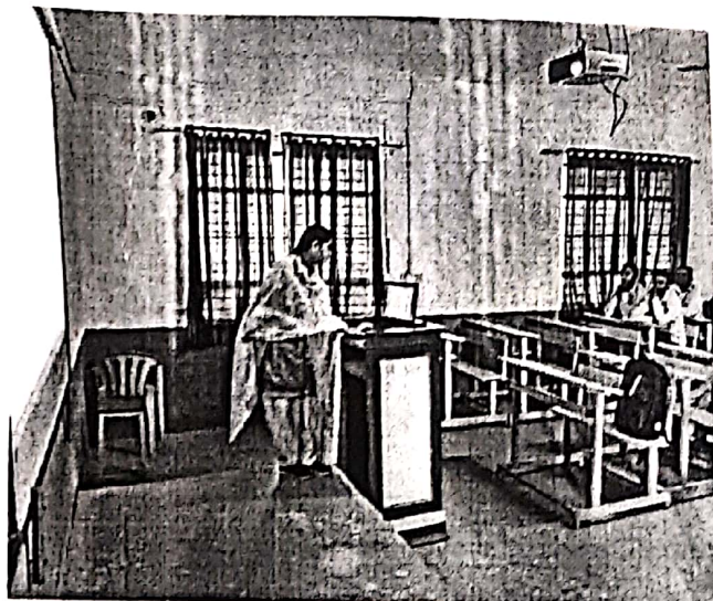
CHEMDRAW LECTURE 2017-18.
