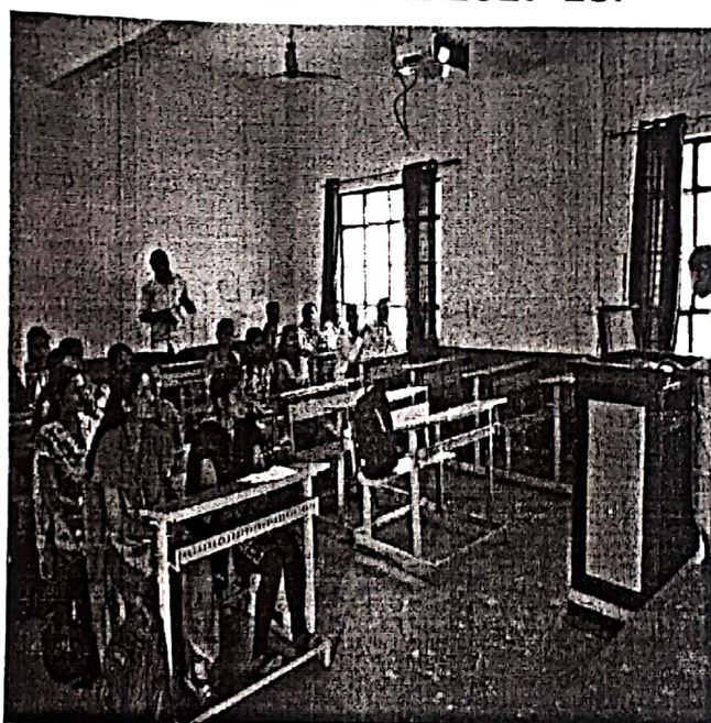
CHEMDRAW LECTURE 2017-18.
